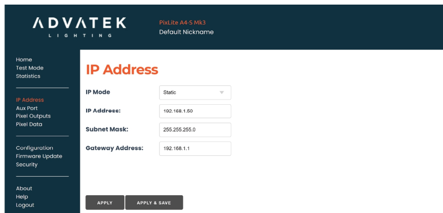
Figure 3: IP Address Configuration with the Management Interface
