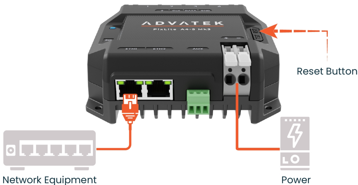
Figure 1: Connection Points & Reset Button
